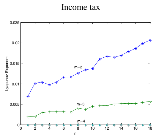
Figure 1. Lyapunov Exponent of taxes time series in different dimensions
