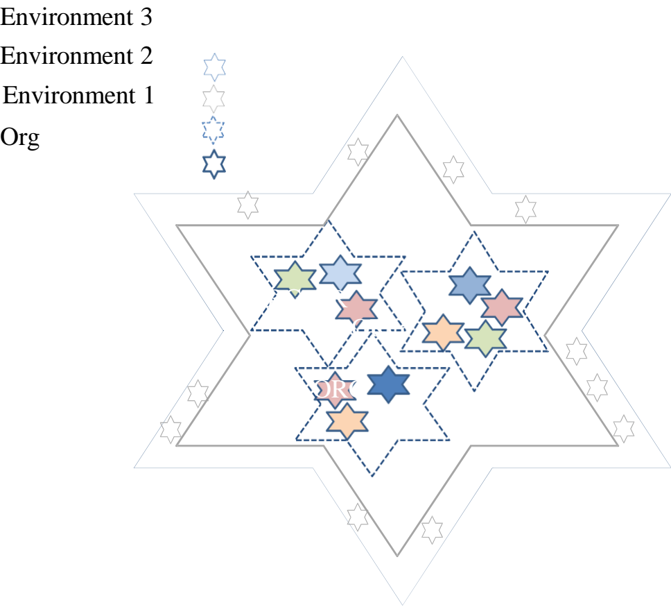
Figure 2. Fractal population ecology theory
